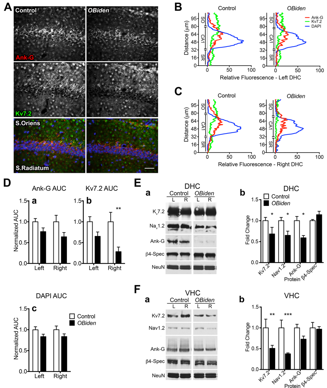
Figure 6. Ion channel disruptions in AIS of hippocampal CA1 neurons. (A) Immunofluorescence labeling for Ank-G (red) and Kv7.2 (green) in the CA1 from control and OBi dorsal hippocampus (DHC). DAPI (blue) shows nuclei. (B,C) Fluorescence intensity plots for each marker in (A) across the left (B) and right (C) DHC CA1. Measurements are orthogonal to CA1 along a 107 \mu m trace from stratum radiatum (SR) to stratum oriens (SO) ( n = 5 mice, 3 slides/mouse). (D) Areas under the curves (AUC) in (B) and (C) for (a) Ank-G, (b) Kv7.2 and (c) DAPI. Kv7.2 intensity in the right DHC CA1 region from OBi mice is reduced compared to controls (two-way RM-ANOVA, genotype \times hemisphere, p < 0.008 , n = 5 ). (E) Representative western blots of DHC punches from control and OBi mice for AIS proteins (a) and quantification (b) shows significant reductions in Ank-G, Kv7.2 and Nav1.2 in OBi mice (two-way RM-ANOVA, genotype \times AIS protein, p < 0.05 , n = 4 ). (F) Representative western blots of left and right ventral hippocampus (VHC) from control and OBi mice for AIS proteins (a) and quantification (b) shows reduced Kv7.2 and Nav1.2 in OBi mice (two-way RM-ANOVA, genotype \times AIS protein, p < 0.01 , n = 4 ). Scale bar in A, 50 \mu m. Abbreviations: \beta 4-Spec, \beta 4-spectrin; Ank-G, ankyrin-G; NeuN as loading control. See unprocessed western blots in Supplementary Information.
